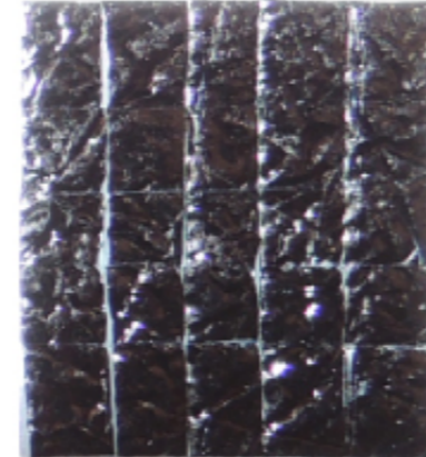
(c) EMIMBF4-FDBC
